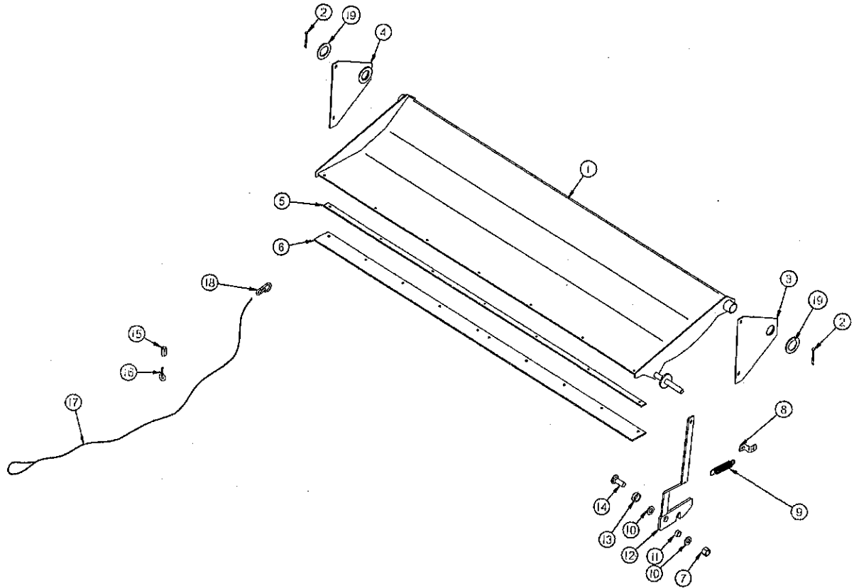
FIGURE 15 H&S HP425 & HP550 SPREADERS OPTIONAL REAR PAN
