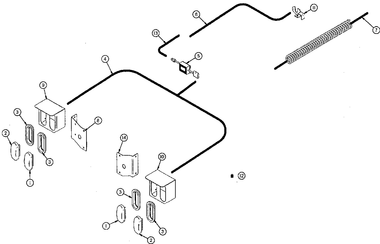
FIGURE 14 H&S HP425 & HP550 SPRADERS OPTIONAL LIGHTING
