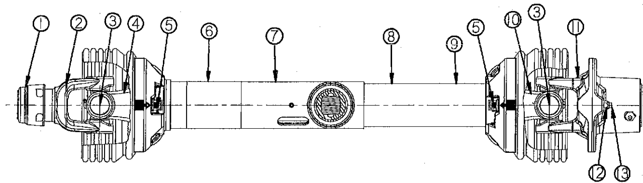
FIGURE 12 H&S HP425 & HP550 SPREADERS PTO & OVERRUNNING CLUTCH
